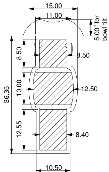
Shroud Bottom
